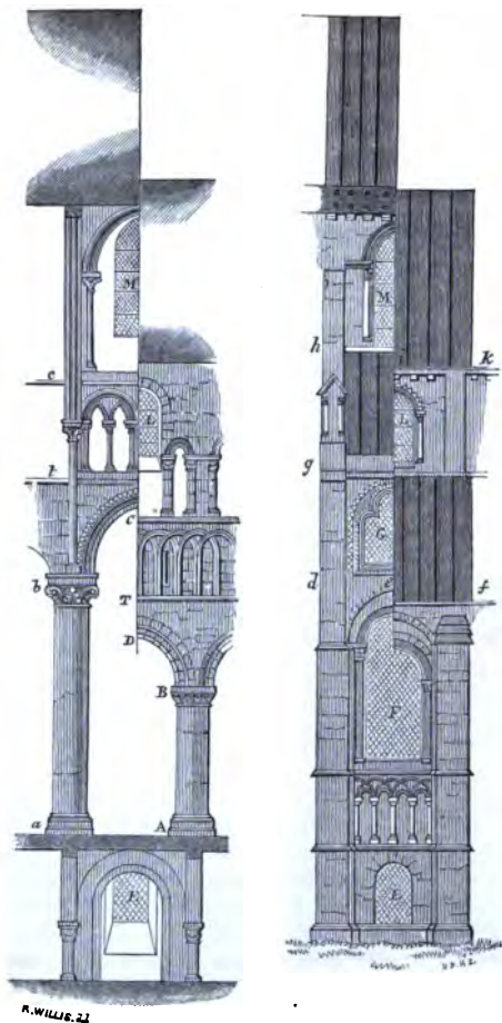
64. Canterbury Cathedral. Exterior and Interior Elevations of the Compartments of the Choir, shewing the changes between A.D. 1066—1130; and 1173—1178.
